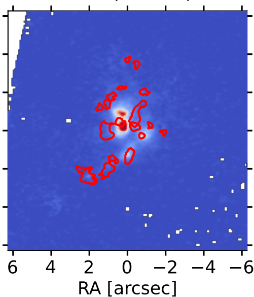
Pa \alpha map - clumps
