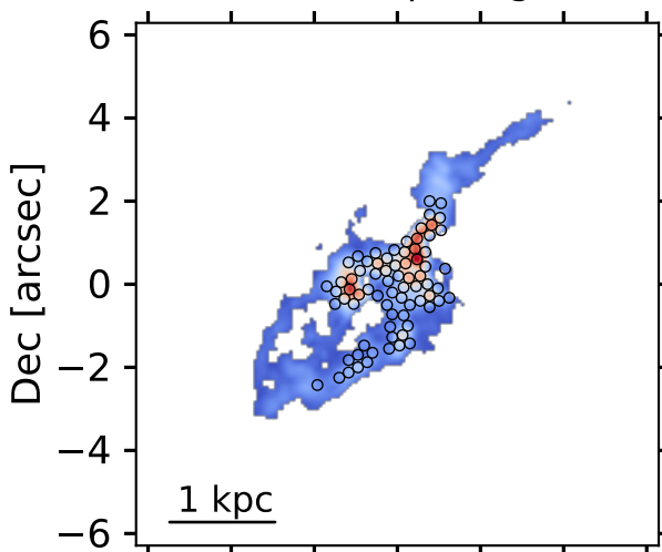
CO(2-1) map - regions
