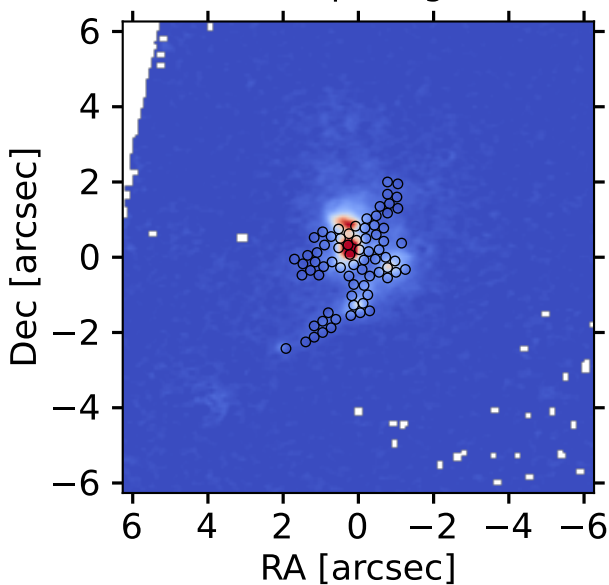
Pa \alpha map - regions
