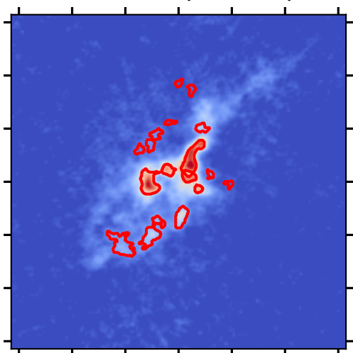
CO(2-1) map - clumps
