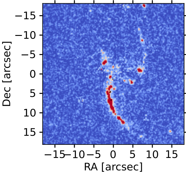
Pa \alpha map - regions
