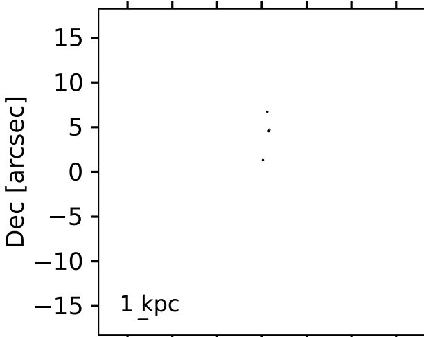
Pa \alpha map - regions
