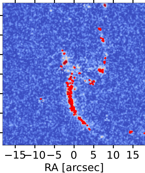
Pa \alpha map - clumps
