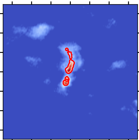
CO(2-1) map - clumps
