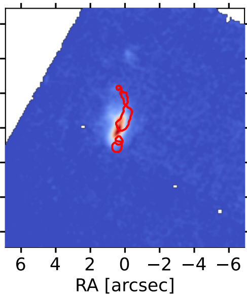
Pa \alpha map - clumps
