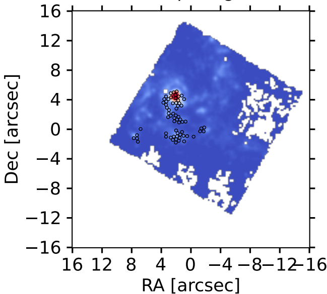
Pa \alpha map - regions
