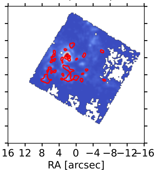
Pa \alpha map - clumps
