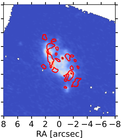
Pa \alpha map - clumps
