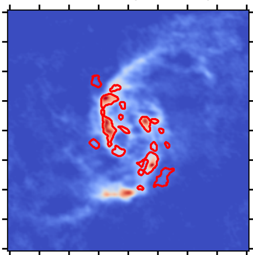
Pa \alpha map - clumps
