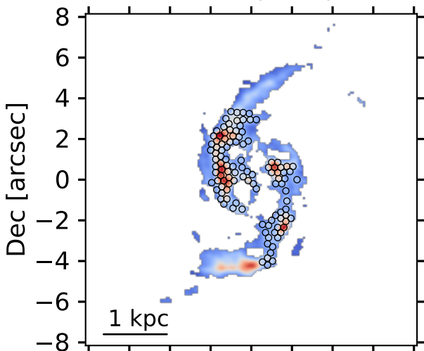
Pa \alpha map - regions
