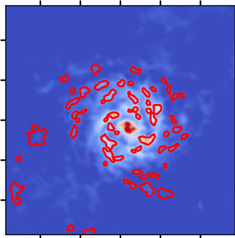
Pa \alpha map - clumps
